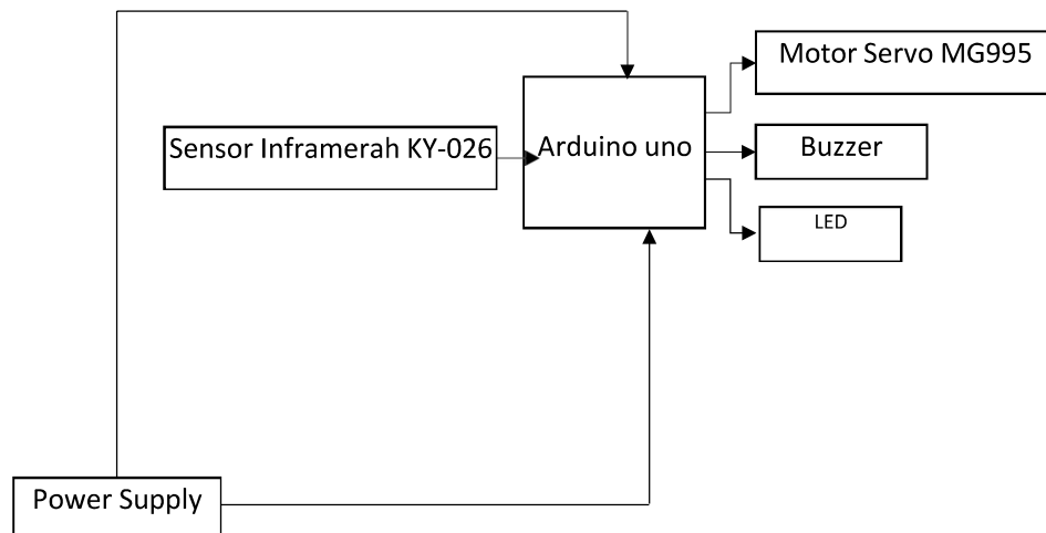
Gambar 3.5 Diagram Block
